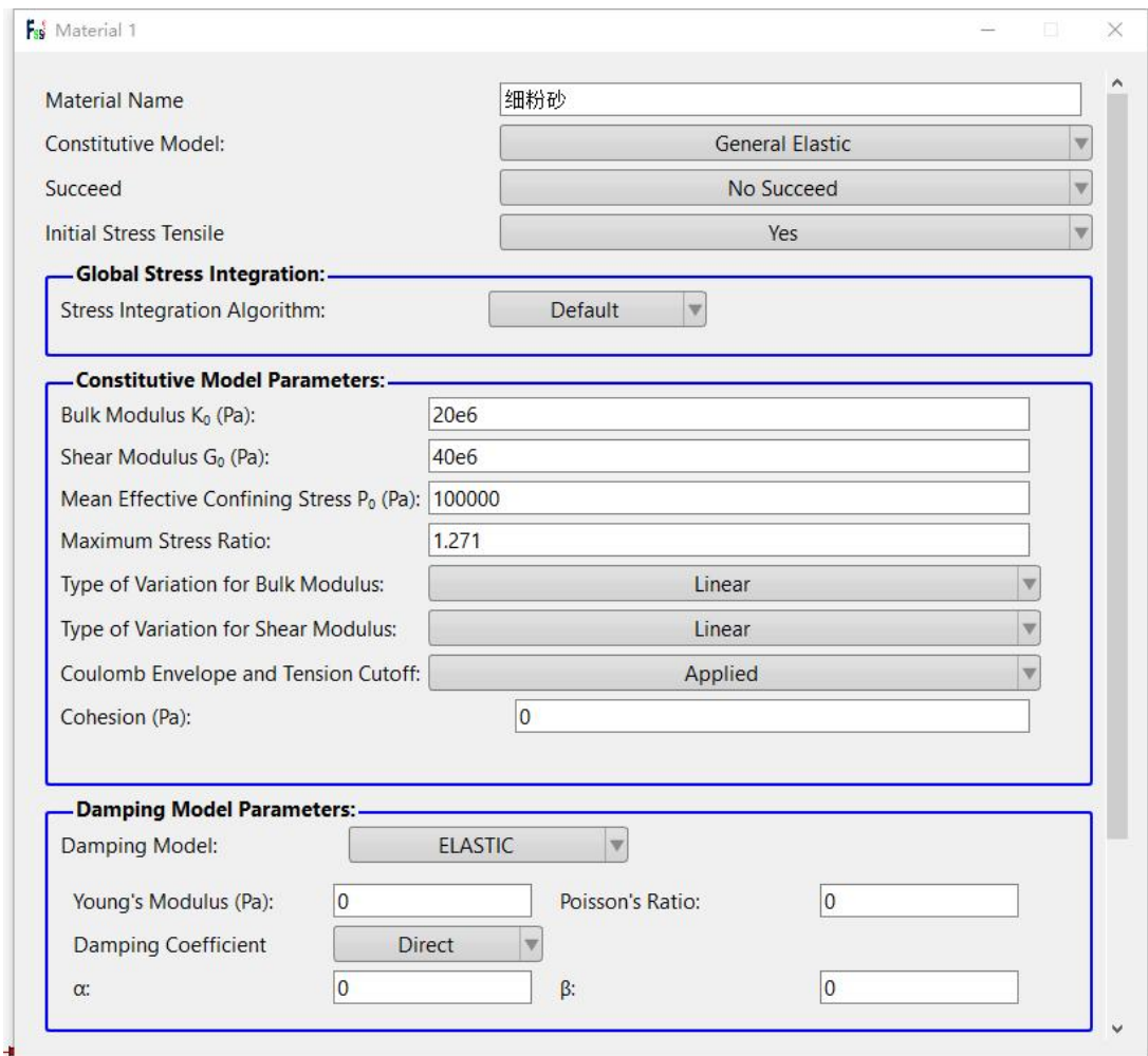
(Material 1 - 粉细砂 )
